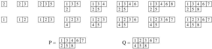
Fig. 2. Construction of the RSK correspondence \text{RSK}(\sigma) = (P, Q) for \sigma = (2, 3, 5, 1, 4, 6, 8, 7) .
