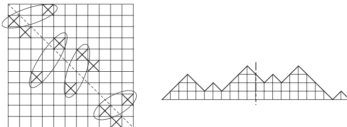
Fig. 5. Example of the matching for \sigma = (4, 1, 2, 5, 7, 8, 3, 6, 11, 9, 10) , and \Psi(\sigma) .
