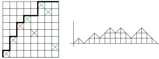
Fig. 3. The bijection \Phi : (6, 7, 4, 3, 5, 2, 8, 1) \mapsto \text{uduuduududdduddd} .
