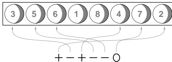
Figure 2: A permutation and its code
