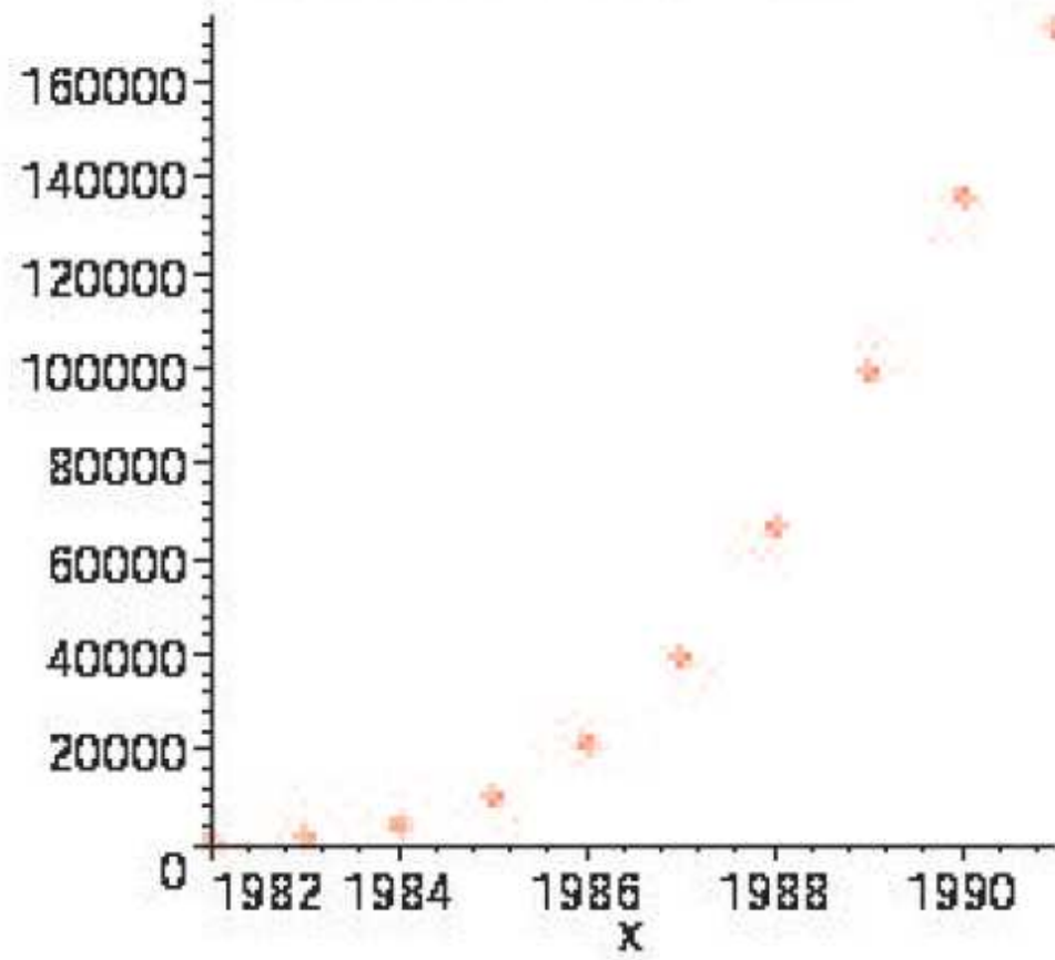
Plot of the AIDS data
