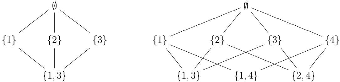
FIGURE 1. Sparse subsets under \preceq
